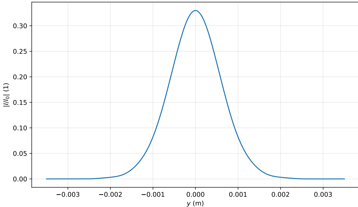
Intensity profile I(x=0, y, z=3.981)/I_0 , P_{in}=0.4P_{cr} , artificial time
